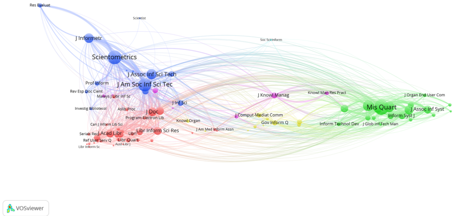
Fig. 4 Clustering of the LIS set ( n = 86 ) into five clusters using VOSviewer
